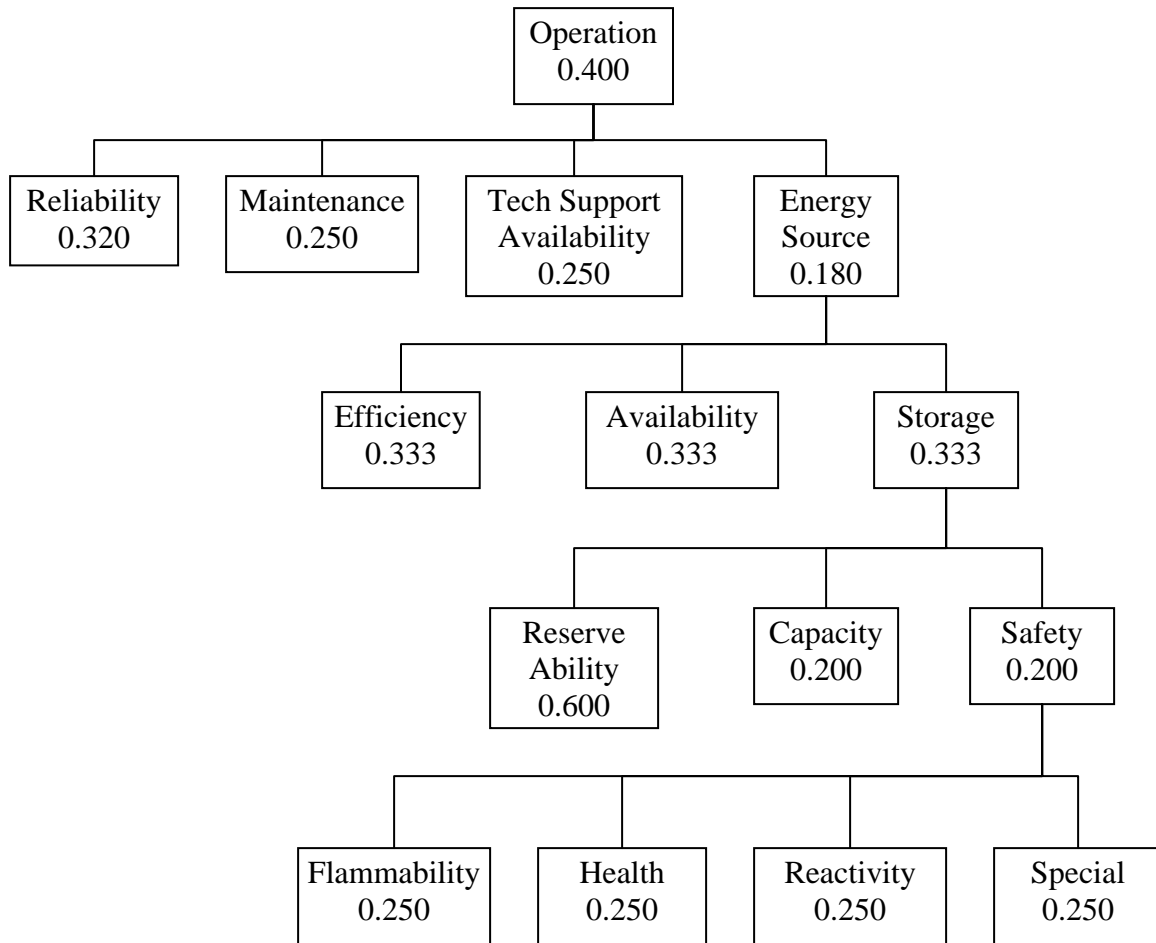
Figure 19. Local Weights-Operation
